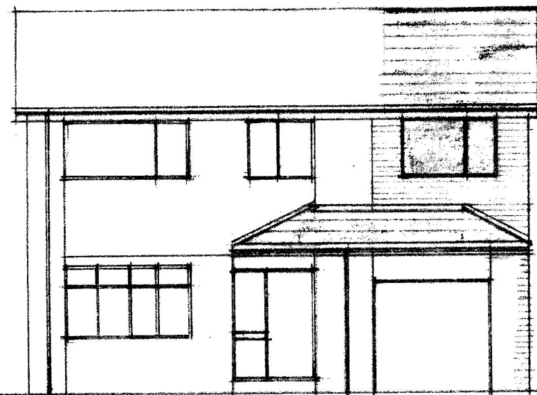
FRONT ELEVATION
